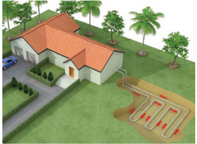
Figure A: Horizontal installation of ground source heat pump. Shallow excavation.
